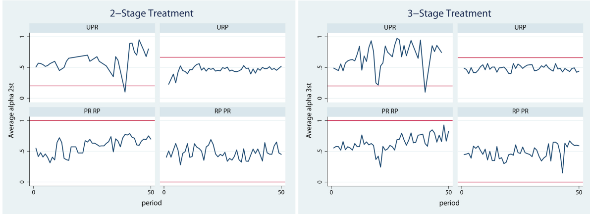
Figure 3: Evolution of incentive parameter by contract combination.
